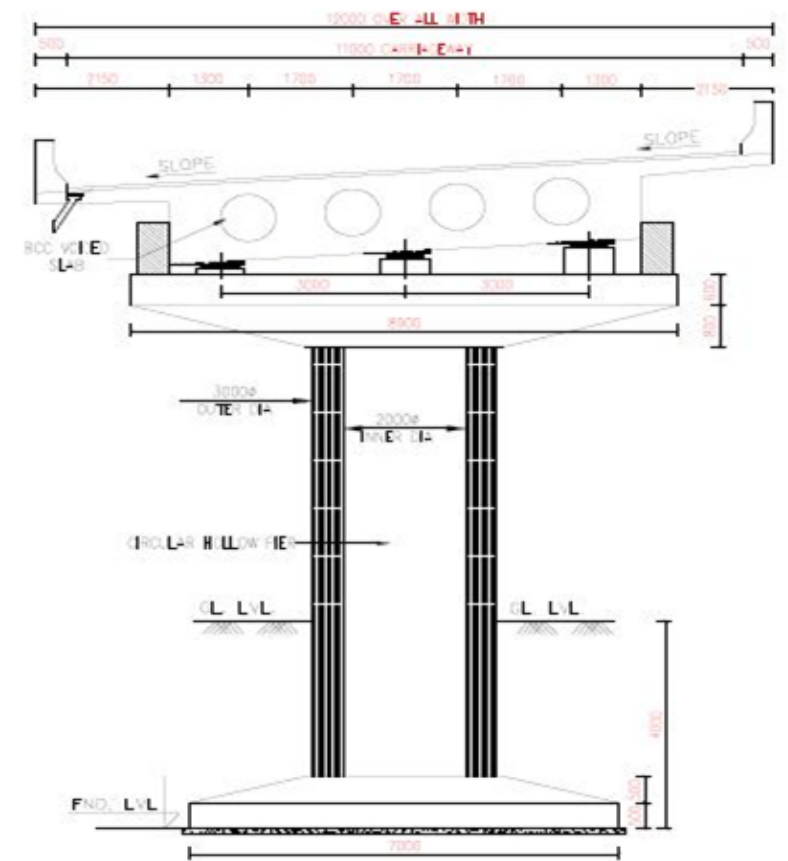
TCS-IX TYPICAL CROSS SECTION FOR ELEVATED STRUCTURE (Including Box Abutment Length)
