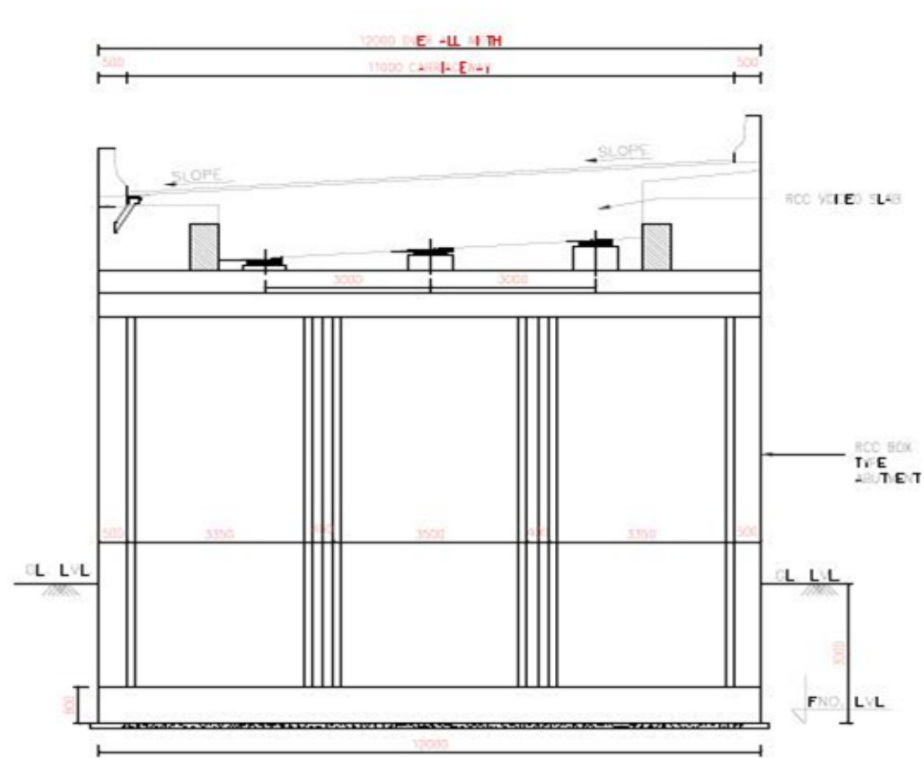
TCS-IX TYPICAL CROSS SECTION FOR ELEVATED STRUCTURE (Including Box Abutment Length)
